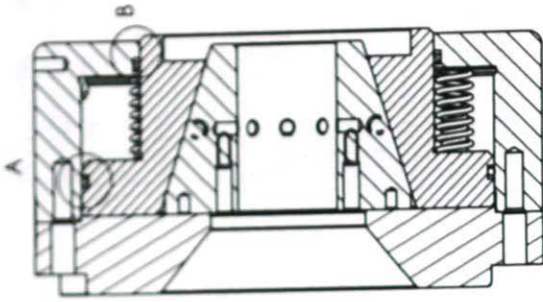
Section view
